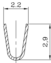
SEC. A-A'
