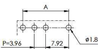
Straight Type
