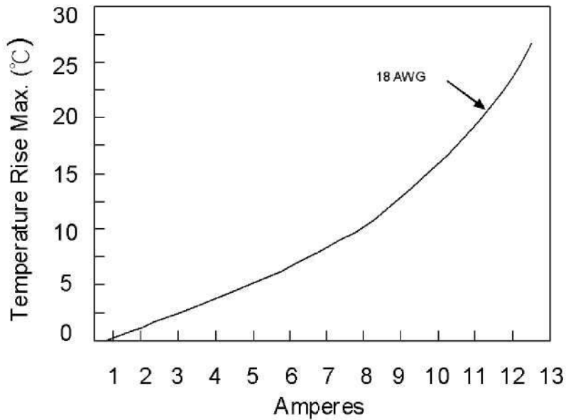
TEMPERATURE RISE CURVE
