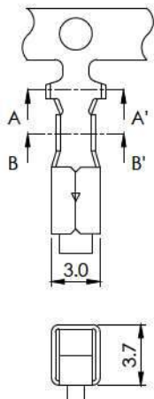
SEC. B-B'
