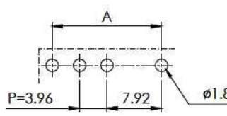
Right-Angle Type
