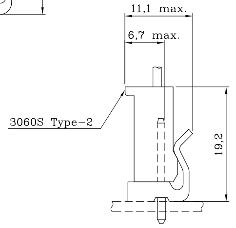
ASSEMBLY LAYOUT
