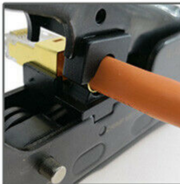
7. crimp the metal clip
