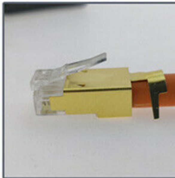
4. close it by hand or by plier the clip close to cable
